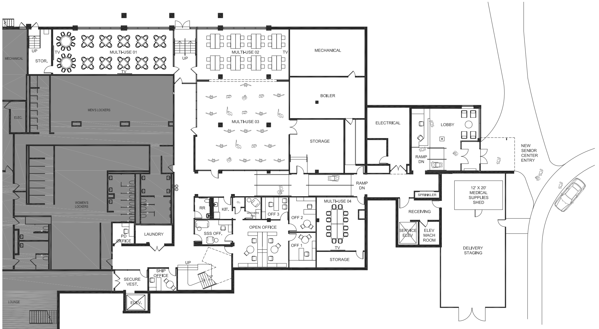
LOWER LEVEL | SENIOR CENTER LAYOUT
